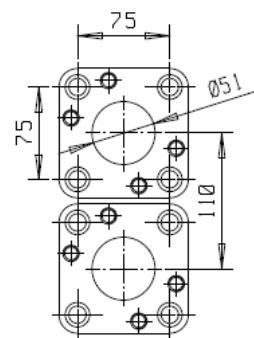
Adapter dimensions SAE 2"-3000M
